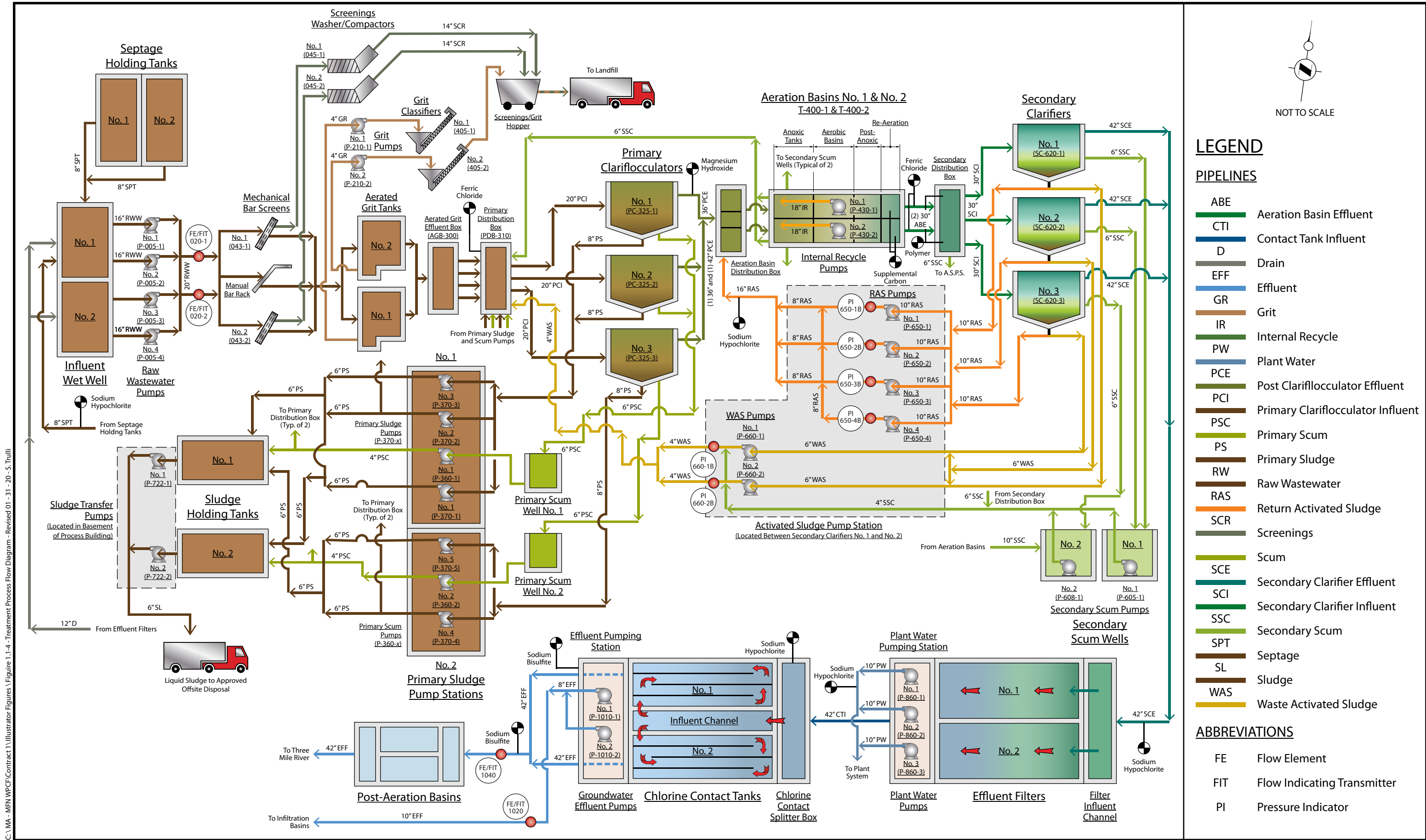
Figure 1.1-4 Treatment Process Flow Diagram
